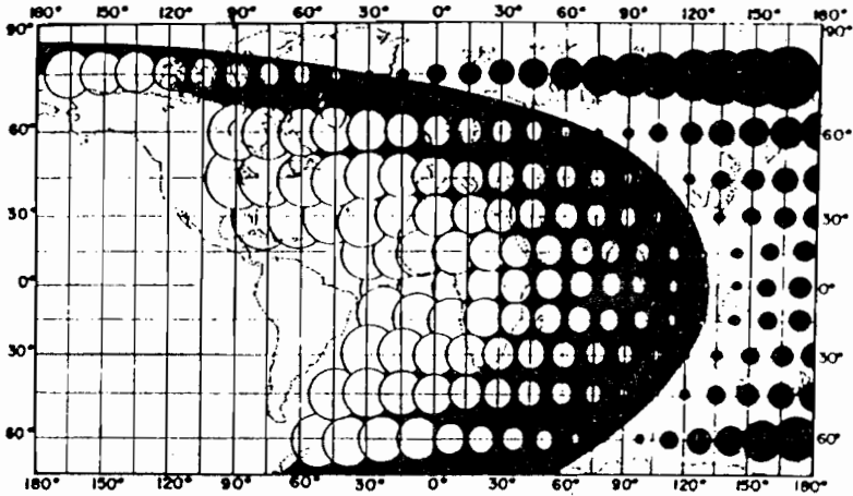
Fig. 1 Schematically illustrates how along the latitude circles, the probability of visibility decreases to the east of IDL (growing dark circles) and increases to the west of IDL (growing white circles).
